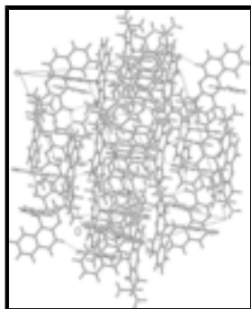
Fig. 2. The packing, showing hydrogen-bond interactions as dashed lines; H atoms are shown as small spheres of arbitrary radii.
